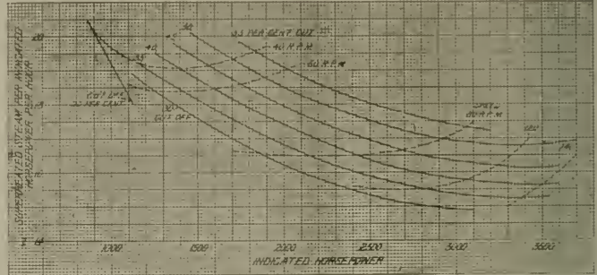
WATER RATES AT ALL CUT OFFS FOR 11S LOCOMOTIVE.
